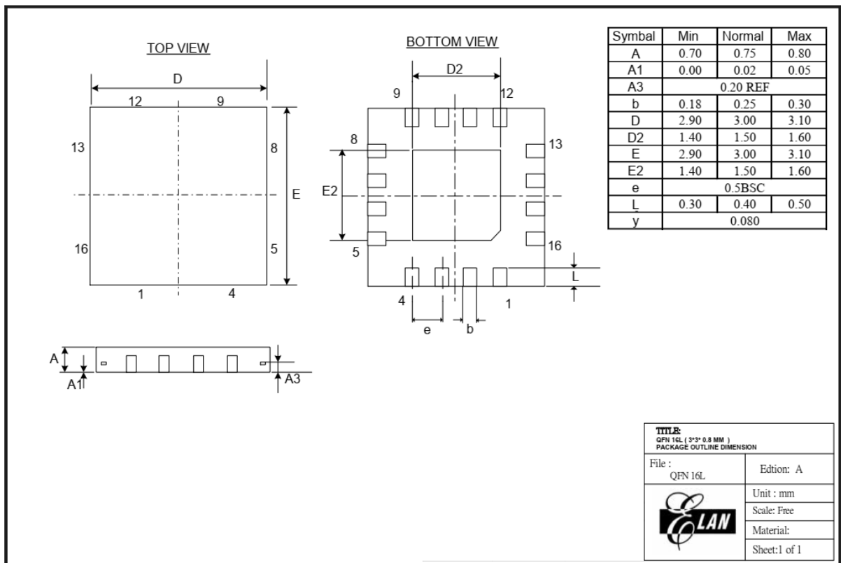
Figure B-2 eKTF6708 16-pin QFN Package Type
