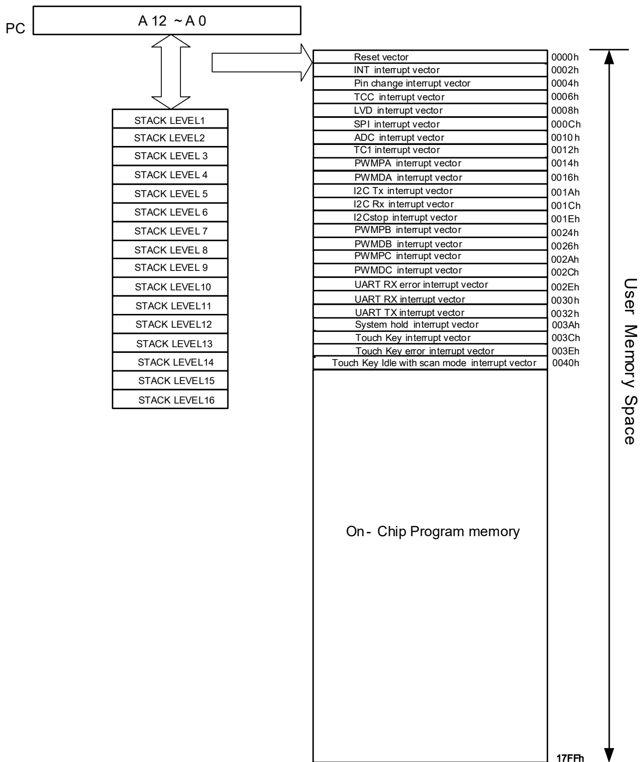
Figure 6-1 eKTF6708 Program Counter Organization
