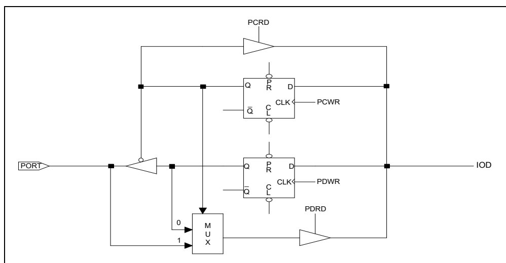
Figure 6-4a I/O Port and I/O Control Register for Port 5~7 Circuit Diagram
