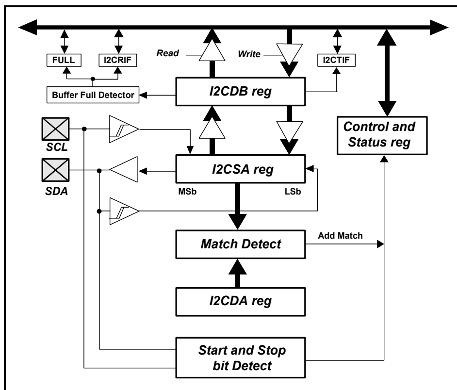
Figure 6-11 eKTF6708 I 2 C Block Diagram
