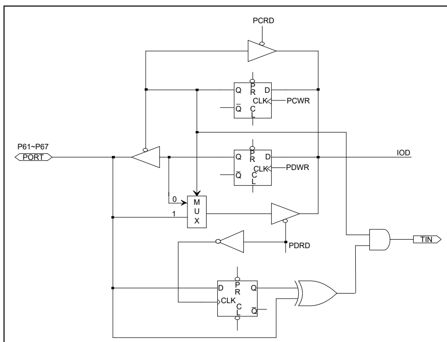
Figure 6-4c I/O Port and I/O Control Register for Ports 5~7 Circuit
