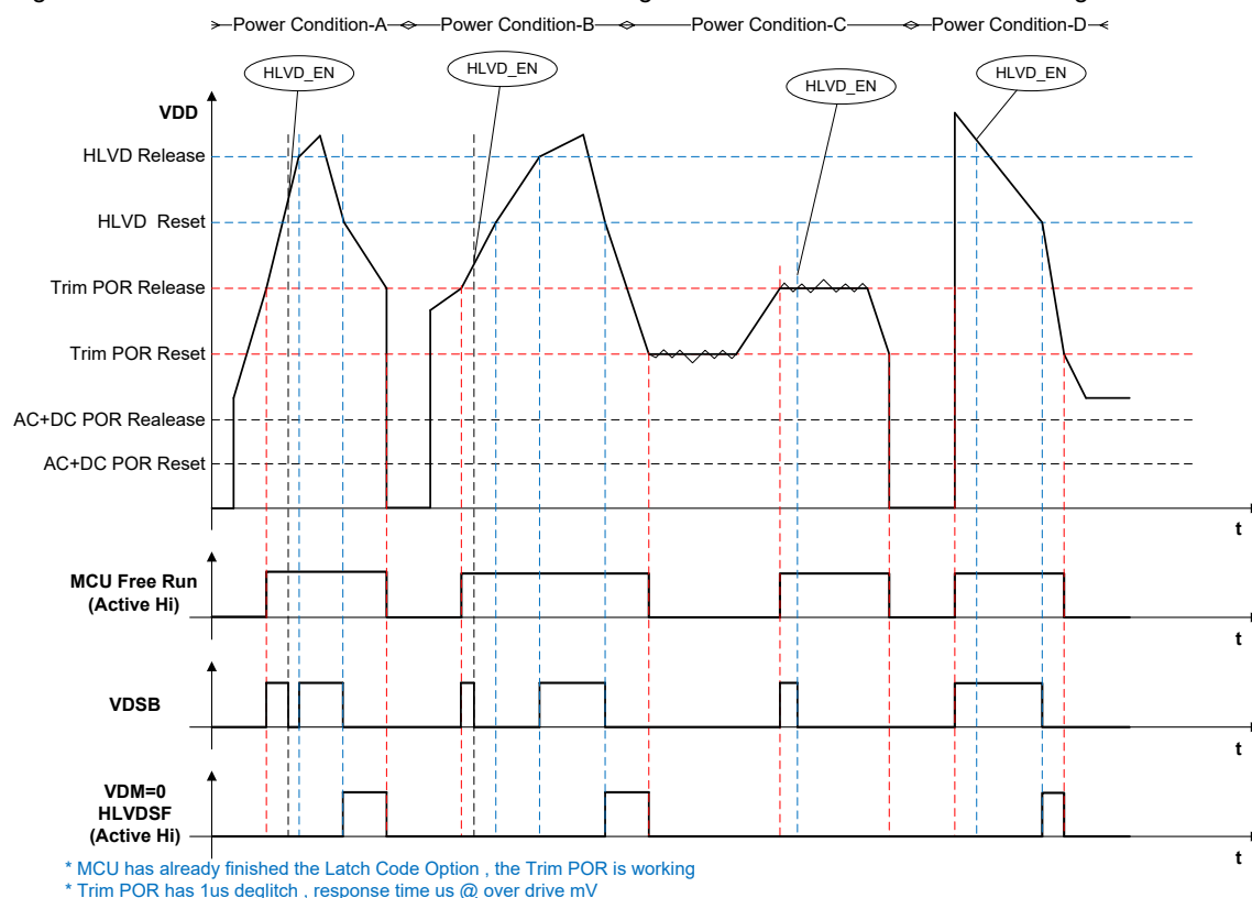
Figure 1.HLVD waveform situation
