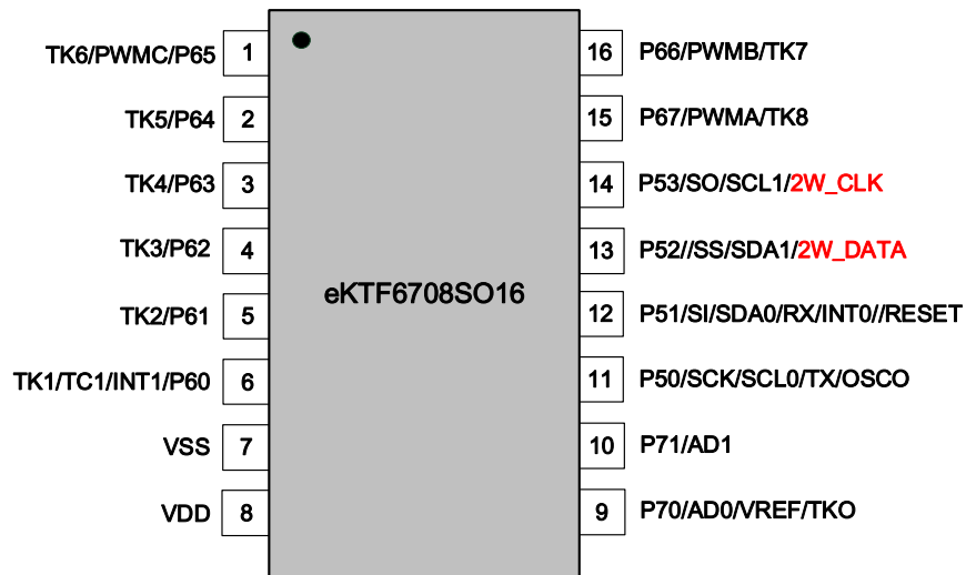
Figure 3-1 SOP-16 Pin Assignment
