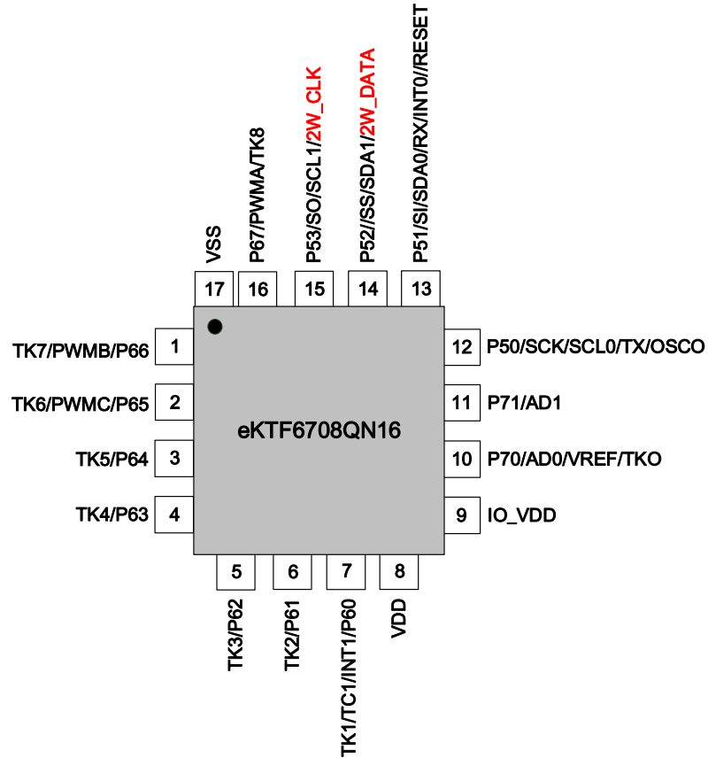
Figure 3-2 QFN-16 Pin Assignment
