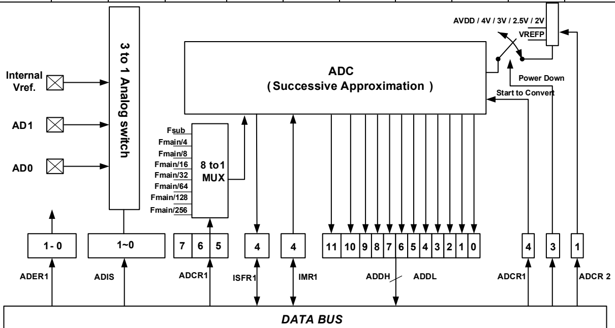
Figure 6-10 AD Converter Functional Block Diagram
