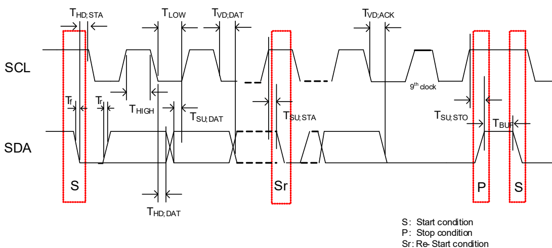
Figure 6-11a eKTF6708 I2C Timing Condition
