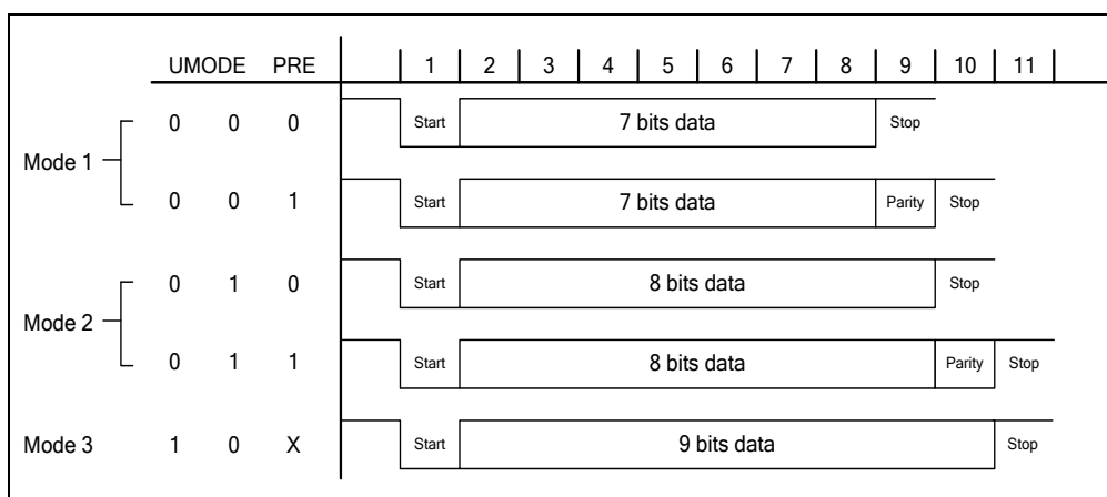
Figure 6-18a UART Model
