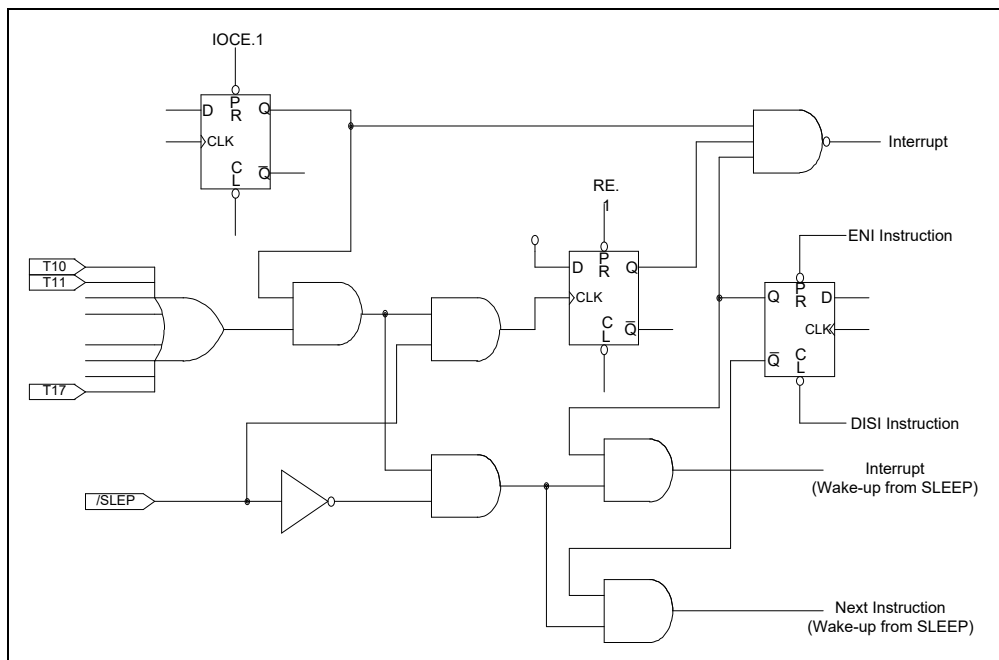
Figure 6-4d I/O Port 5~7 with Input Change Interrupt/Wake-up Block Diagram
