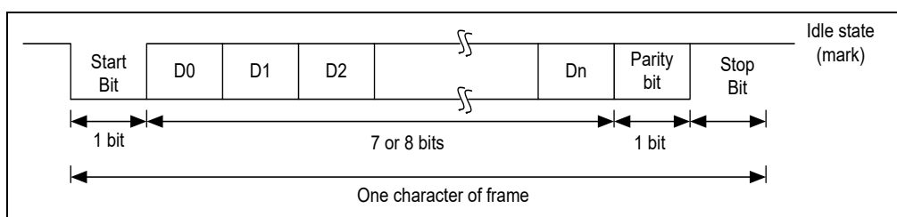
Figure 6-17 Data Format in UART
