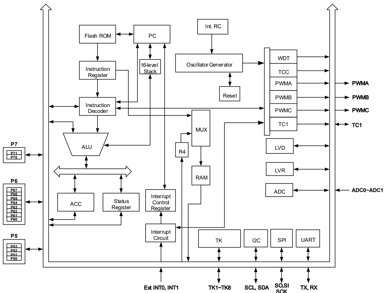
Figure 5-1 eKTF6708 Functional Block Diagram
