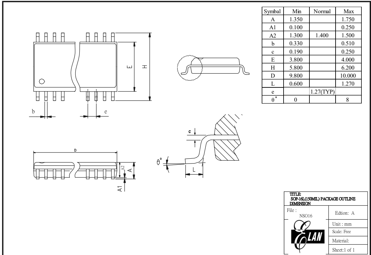
Figure B-1 eKTF6708 16-pin SOP Package Type
